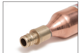
PEX Crimp/Expansion
